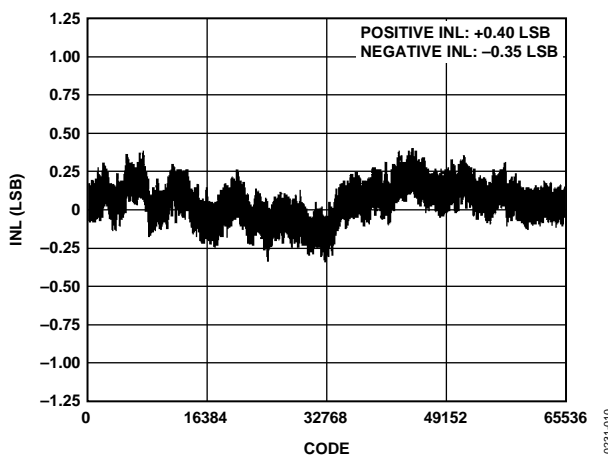
Figure 10. Integral Nonlinearity vs. Code, V_{REF} = 5\text{ V}
