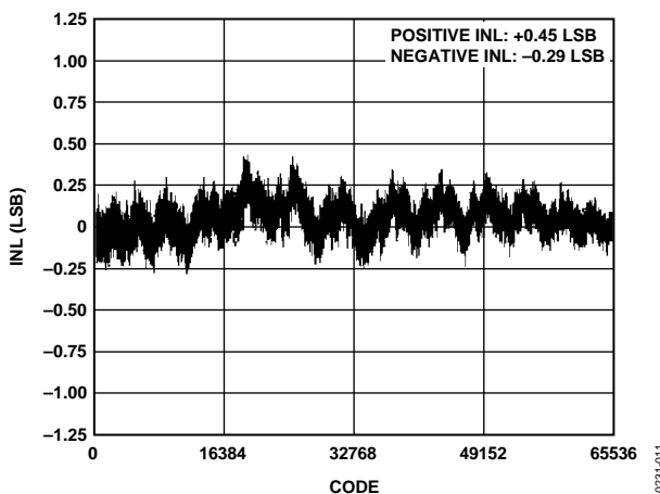
Figure 11. Integral Nonlinearity vs. Code, V_{REF} = 2.5\text{ V}
