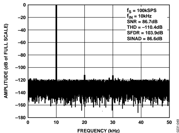
Figure 9. AD7988-1 FFT Plot, V_{REF} = 2.5\text{ V}
