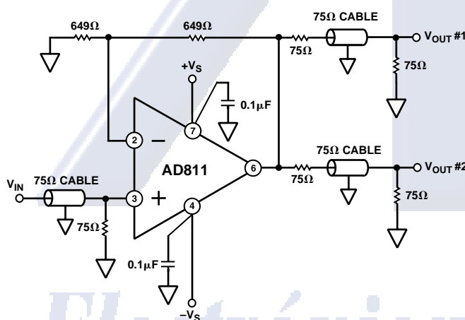
Figure 35. A Video Line Driver Operating at a Gain of +2
