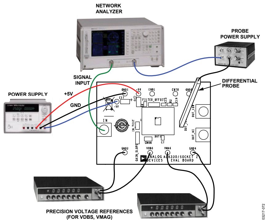
Figure 71. Typical Connections
