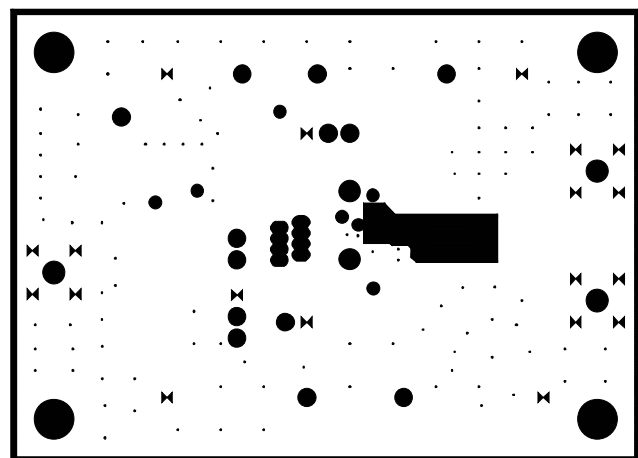
Figure 74. Ground Plane
