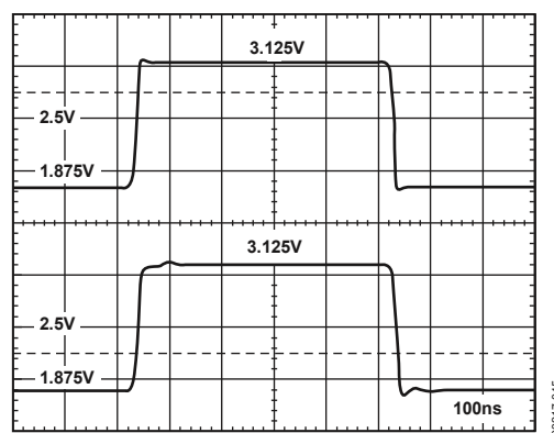
Figure 44. CNTR Transient Response, Top: Input to CNTR, Bottom: V_{OUT} Single-Ended
