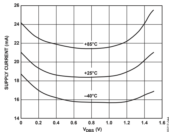
Figure 43. Supply Current vs. V_{DBS} at Three Temperatures
