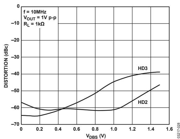
Figure 27. Harmonic Distortion vs. V_{DBS}
