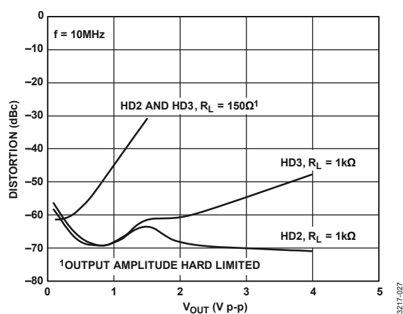
Figure 26. Harmonic Distortion vs. V_{OUT} , V_{MAG} = 2.0 V
