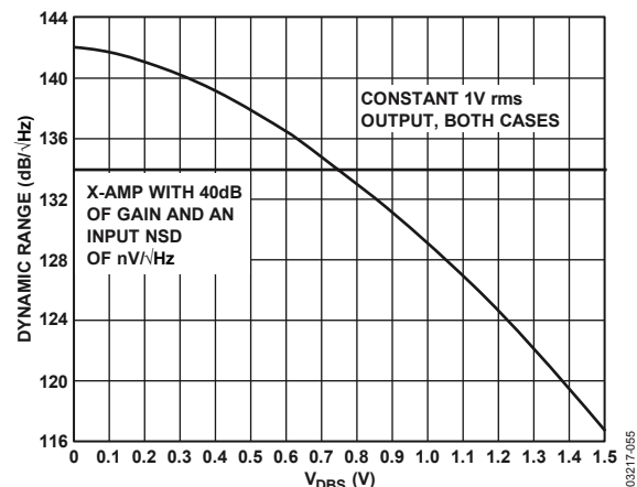
Figure 54. Dynamic Range in dB/√Hz vs. V_{\text{DBS}} ( V_{\text{MAG}} = 0.5 V, 1 V rms Output) Compared with a Representative X-AMP (Simulation)
