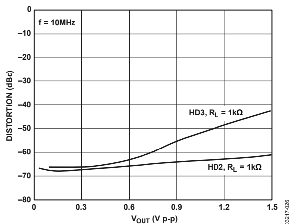
Figure 25. Harmonic Distortion vs. V_{OUT} , V_{MAG} = 0.5 V
