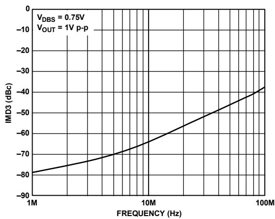
Figure 30. IMD3 Distortion vs. Frequency
