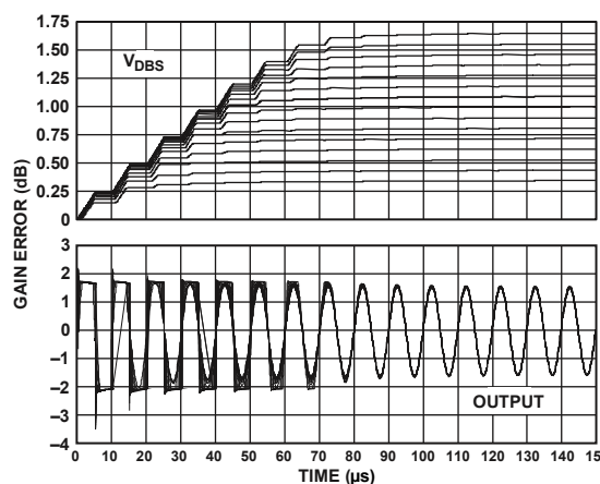
Figure 66. Time Domain Waveforms (Simulation)
