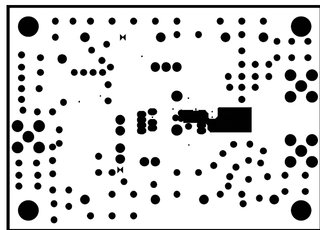
Figure 77. Inner Layer 2
