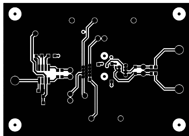
Figure 76. Wiring Side Pattern
