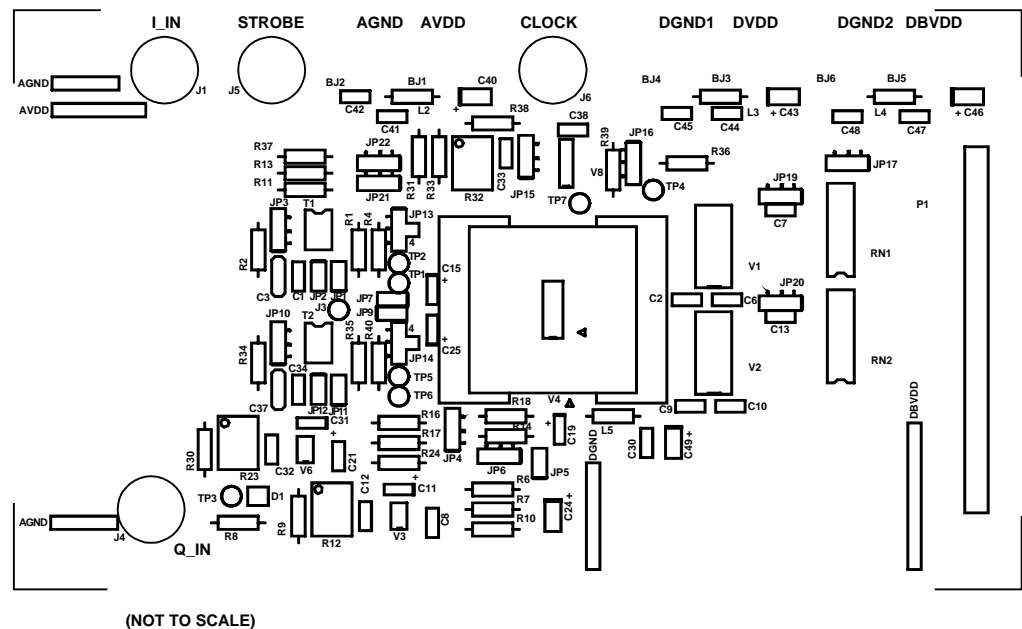
Figure 40. Evaluation Board Component-Side Silkscreen
