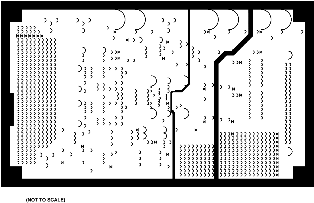
Figure 41. Evaluation Board Power Plane Layout
