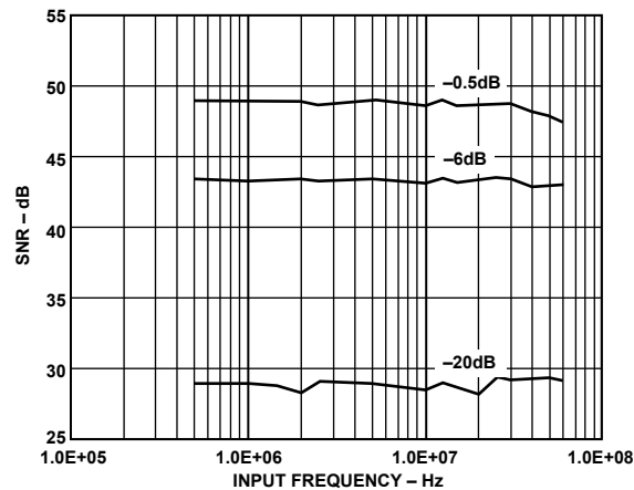
Figure 6. SNR vs. Input Frequency
