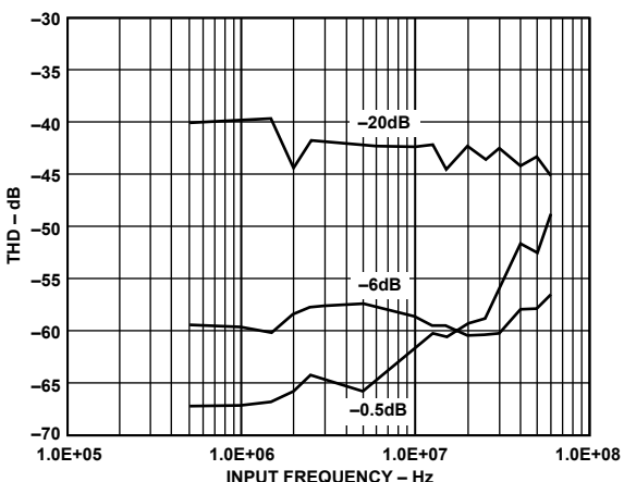
Figure 8. THD vs. Input Frequency
