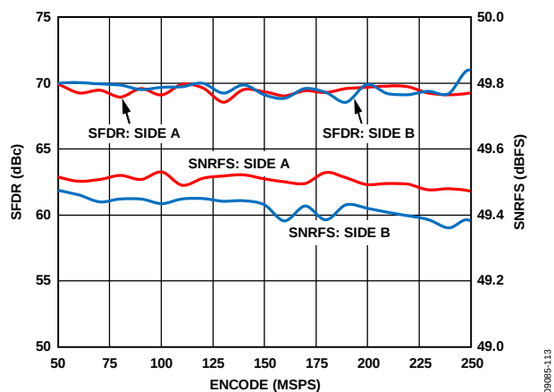
Figure 10. SNRFS/SFDR vs Encode with f_{IN} = 2.4 MHz
