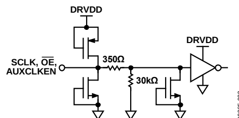
Figure 16. SCLK, OE
