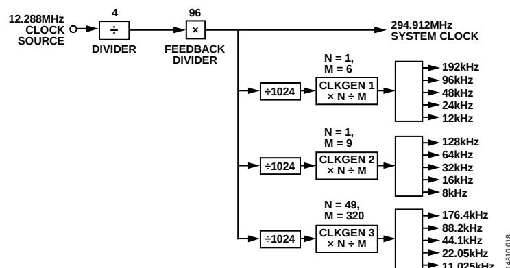
Figure 18. PLL and Audio Clock Generators with Default Settings and Resulting Clock Frequencies Labeled, XTALIN/MCLK = 12.288 MHz
