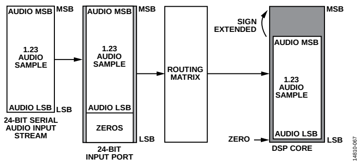
Figure 69. 24-Bit Serial Input Example
