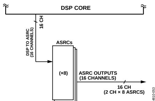
Figure 55. Example ASRC Routing for Asynchronous Serial Output from the DSP Core
