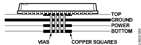
Figure 87. Exposed Pad Layout Example—Side View
