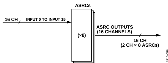
Figure 58. Example ASRC Routing, Bypassing DSP Core
