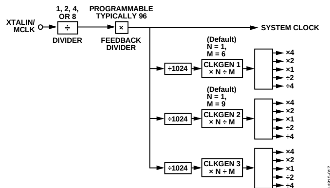
Figure 17. PLL and Clock Generators Block Diagram
