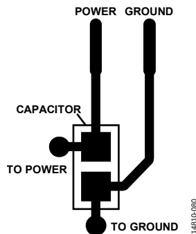
Figure 84. Recommended Power Supply Bypass Capacitor Layout
