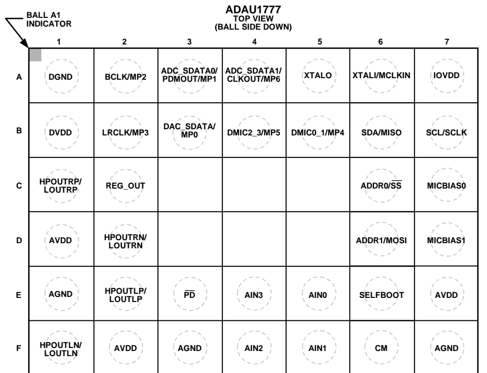
Figure 9. Pin Configuration
