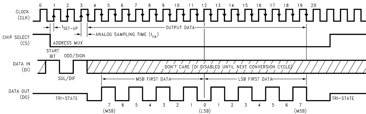
ADC08032 Timing
