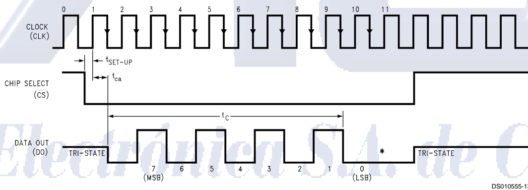
ADC08031 Timing
