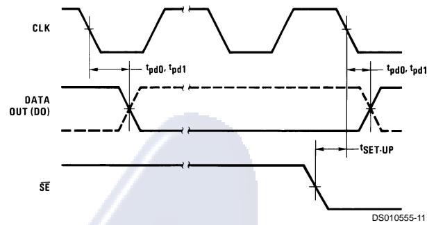
Data Output Timing
