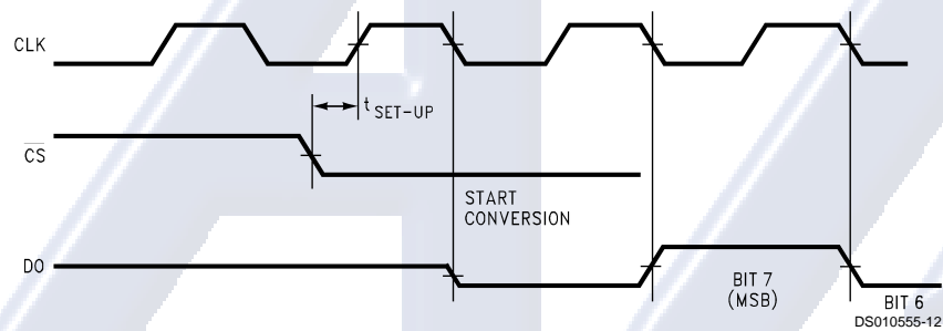
ADC08031 Start Conversion Timing
