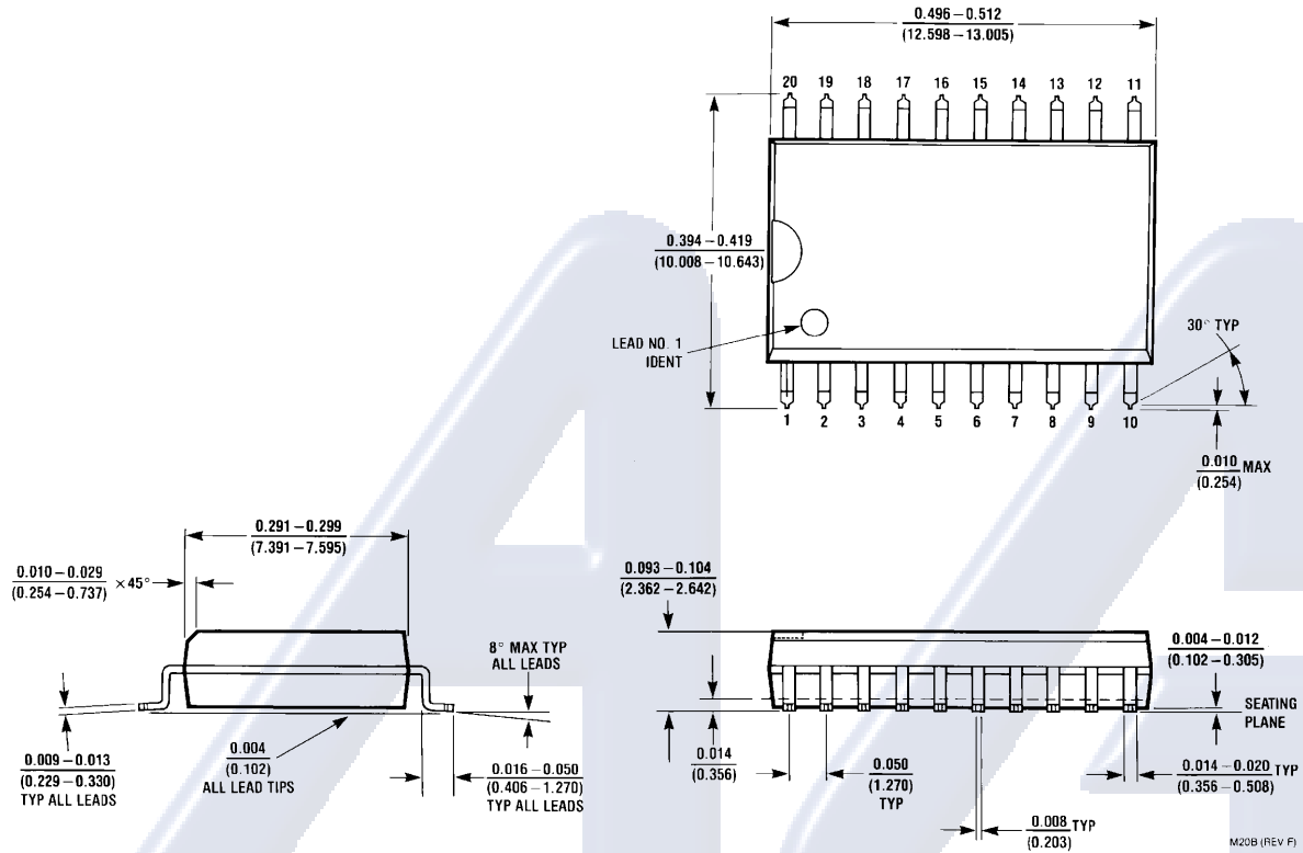
Order Number ADC08038CIWM NS Package Number M20B
