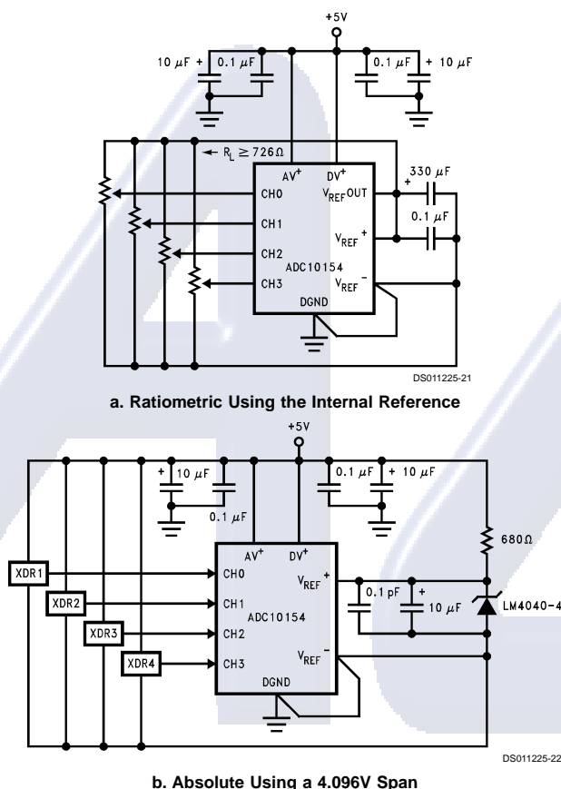
a. Ratiometric Using the Internal Reference b. Absolute Using a 4.096V Span FIGURE 5. Different Reference Configurations
