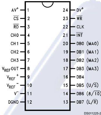
Top View Order Number ADC10154 NS Package Number M24B
