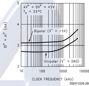
Total Positive Power Supply Current ( I_{I^+} + A_{I^+} ) vs Clock Frequency
