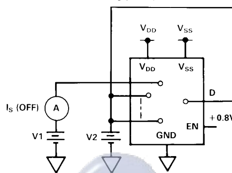
TEST CIRCUIT 2
