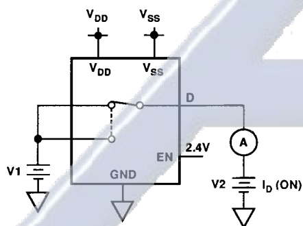
TEST CIRCUIT 4
