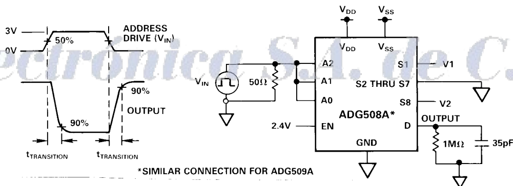
TEST CIRCUIT 7
