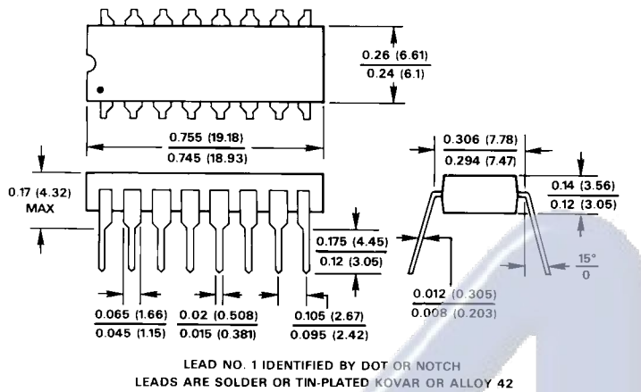
16-Pin Plastic (N-16)
