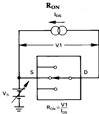
TEST CIRCUIT 4
