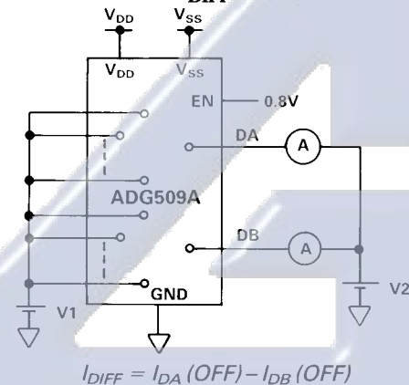
TEST CIRCUIT 5
