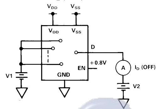
TEST CIRCUIT 5
