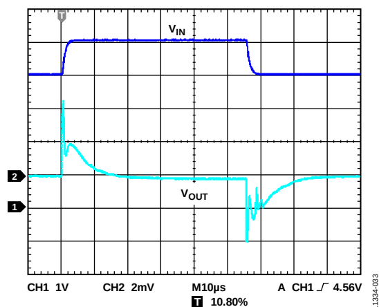
Figure 33. Line Transient Response, C_{IN} and C_{OUT} = 1\ \mu F , I_{LOAD} = 200\ mA
