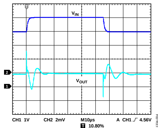
Figure 34. Line Transient Response, C_{IN} and C_{OUT} = 1\ \mu F , I_{LOAD} = 1\ mA
