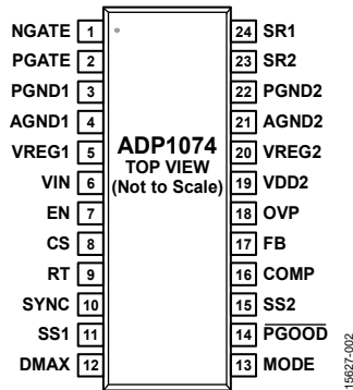
Figure 4. 24-Lead SOIC_W Pin Configuration
