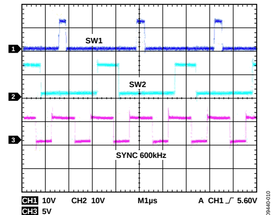
Figure 9. An Example of Synchronization, f_{\text{SYNC}} = 600 \text{ kHz}
