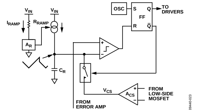
Figure 22. Simplified Control Architecture
