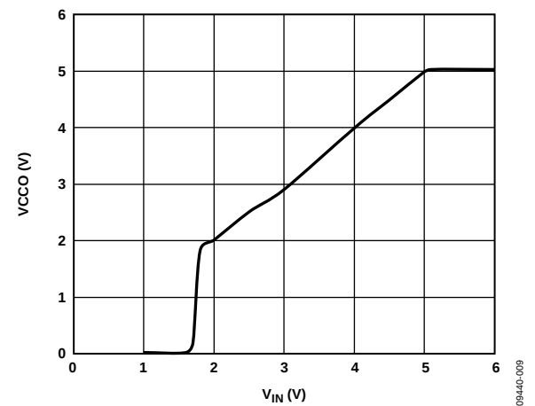
Figure 8. V_O vs. V_{IN}
