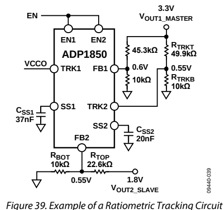
Figure 39. Example of a Ratiometric Tracking Circuit
