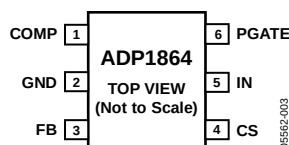
Figure 2. Pin Configuration
