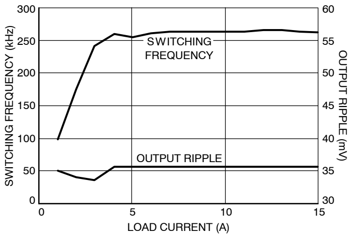
Figure 5. Switching Frequency vs. Load Current in RPM Mode
