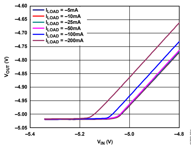
Figure 26. Output Voltage ( V_{OUT} ) vs. Input Voltage ( V_{IN} ) in Dropout, V_{OUT} = -5 V
