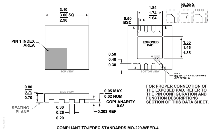
COMPLIANT TO JEDEC STANDARDS MO-229-WEED-4 Figure 105. 8-Lead Lead Frame Chip Scale Package [LFCSP] 3 mm x 3 mm Body and 0.75 Package Height (CP-8-13)
