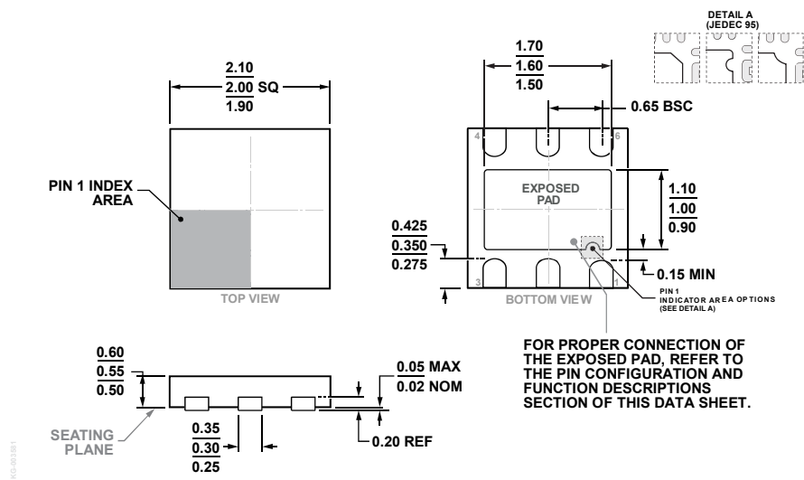
Figure 104. 6-Lead Lead Frame Chip Scale Package [LFCSP] 2.00 mm x 2.00 mm Body and 0.55 Package Height (CP-6-3)
