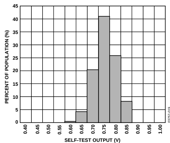
Figure 17. Y-Axis Self-Test Response at 25°C
