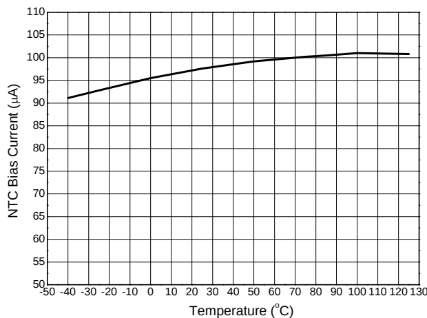
NTC Bias Current vs. Temperature
