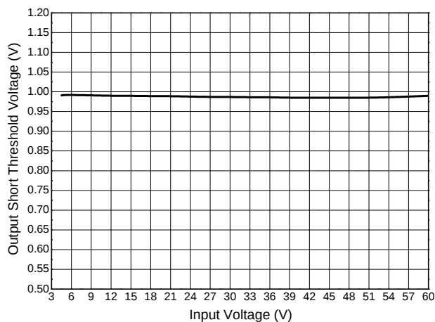
Output Short Threshold Voltage vs. Input Voltage
