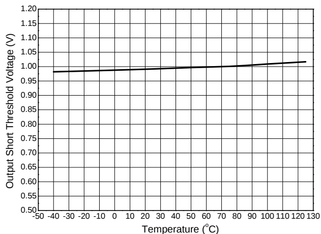
Output Short Threshold Voltage vs. Temperature
