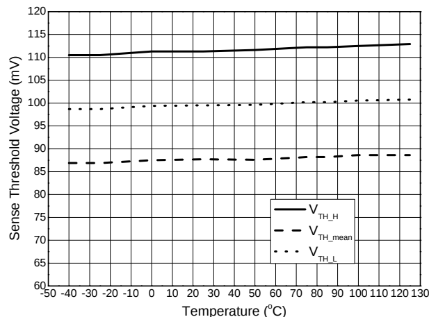
Sense Threshold Voltage vs. Temperature
