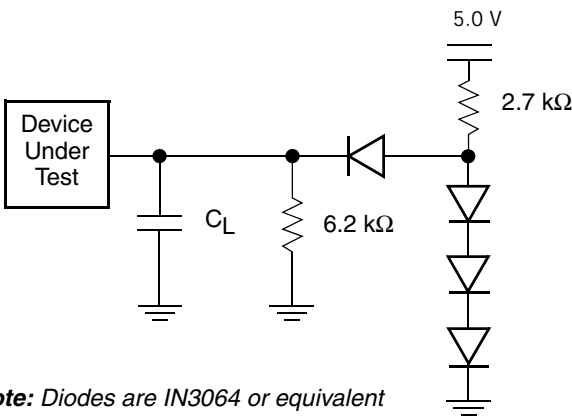
Figure 7. Test Setup
