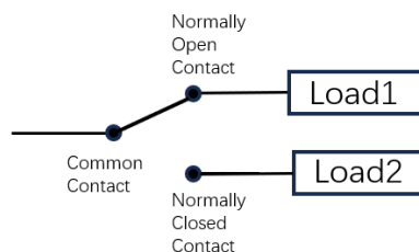
Relay activates if alarm is triggered
