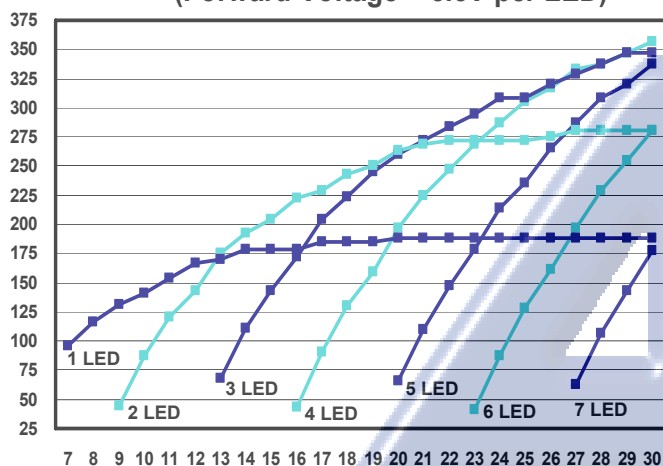
Operating Frequency vs Input Voltage (Forward Voltage = 3.5V per LED)
