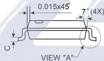
VIEW "A"
