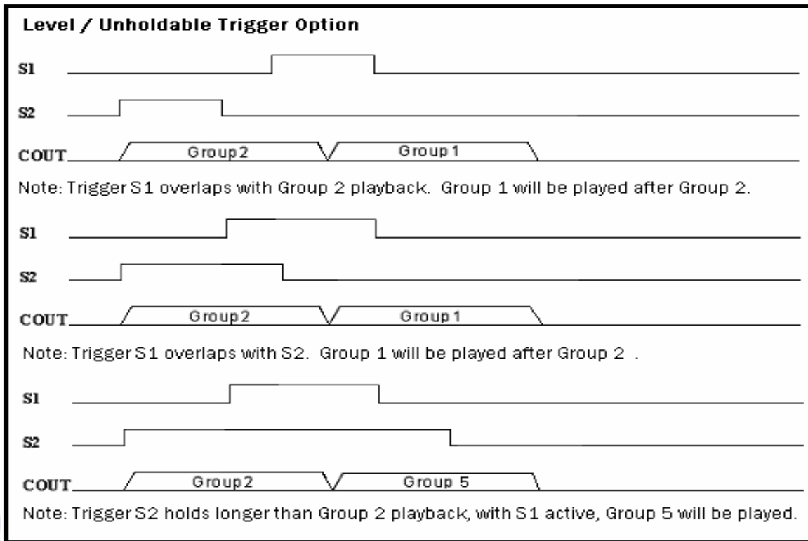
Fig. 10 Overlap trigger
