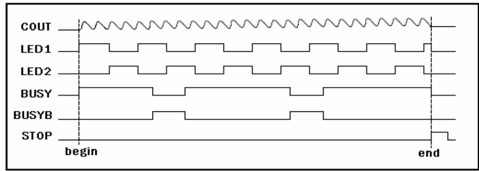
Fig. 3 Output waveforms
