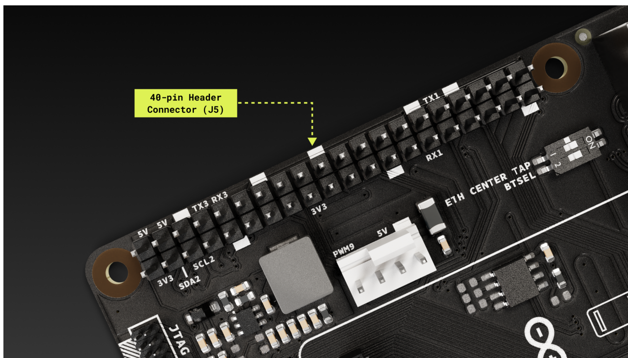
Figure 8. Raspberry Pi®-compatible 40-pin header connector
