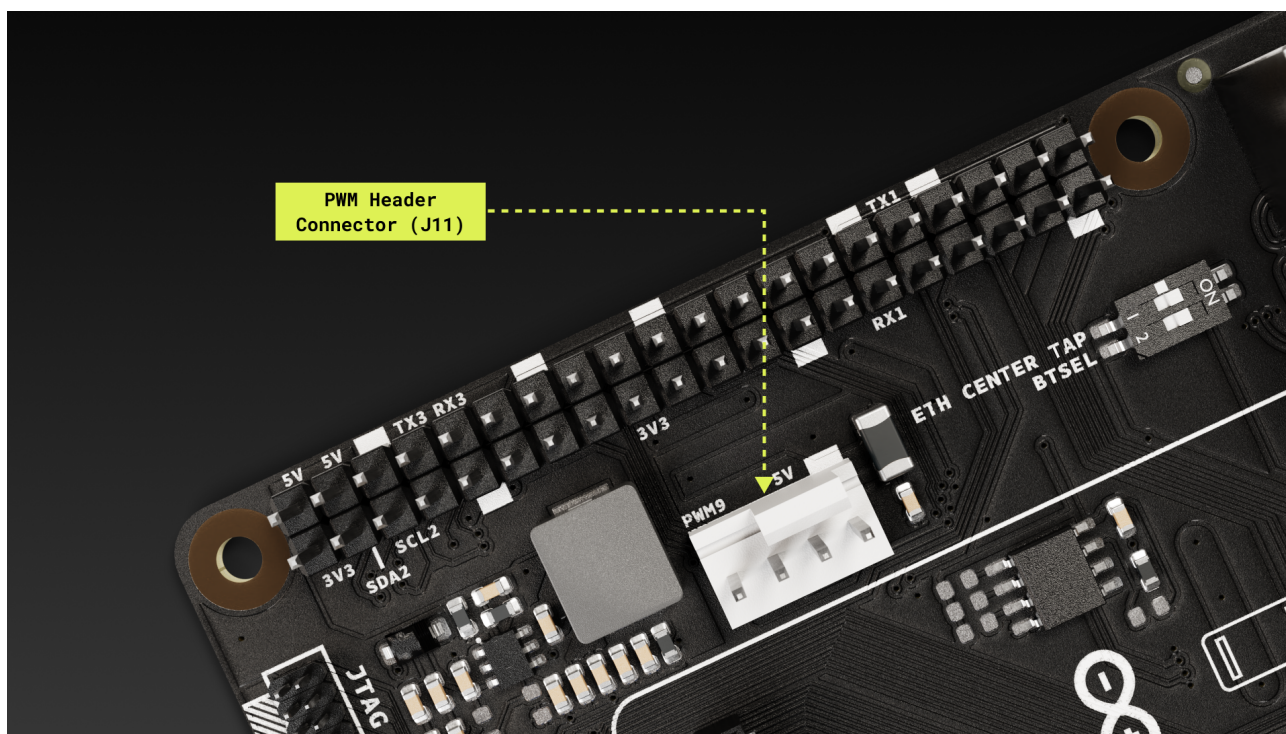
Figure 14. PWM connector of the Portenta Hat Carrier
