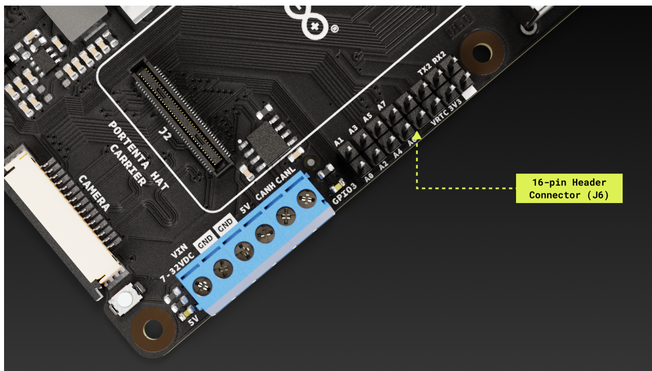
Figure 9. 16-pin header connector
