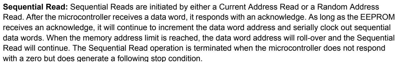
Figure 9-3. Sequential Read
