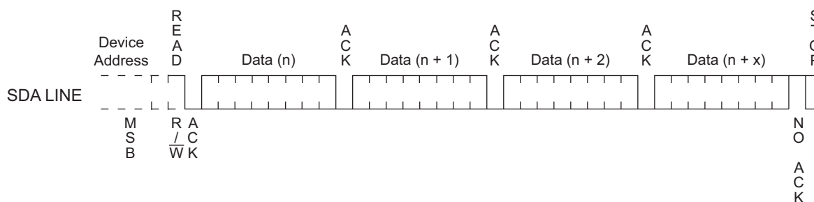
Figure 9-3. Sequential Read
