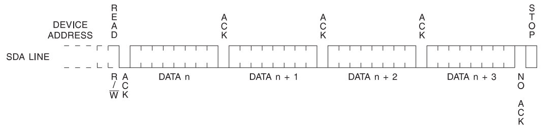
Figure 7-3. Sequential Read
