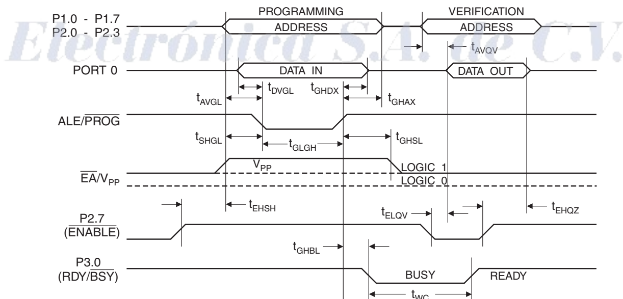
Figure 18-1. Flash Programming and Verification Waveforms – Parallel Mode
