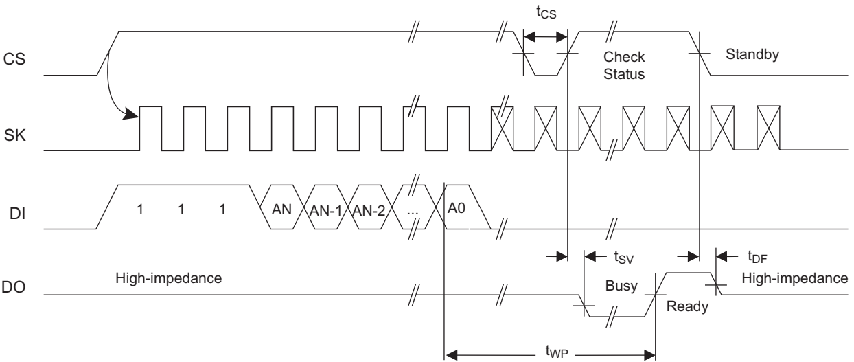
Figure 6-2. ERASE Timing
