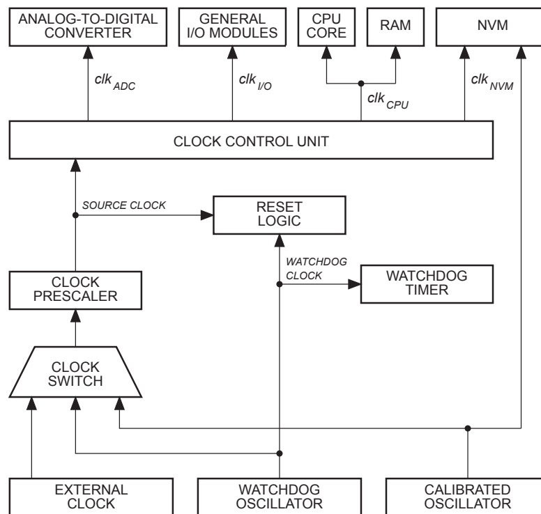
Figure 8-1 Clock Distribution
