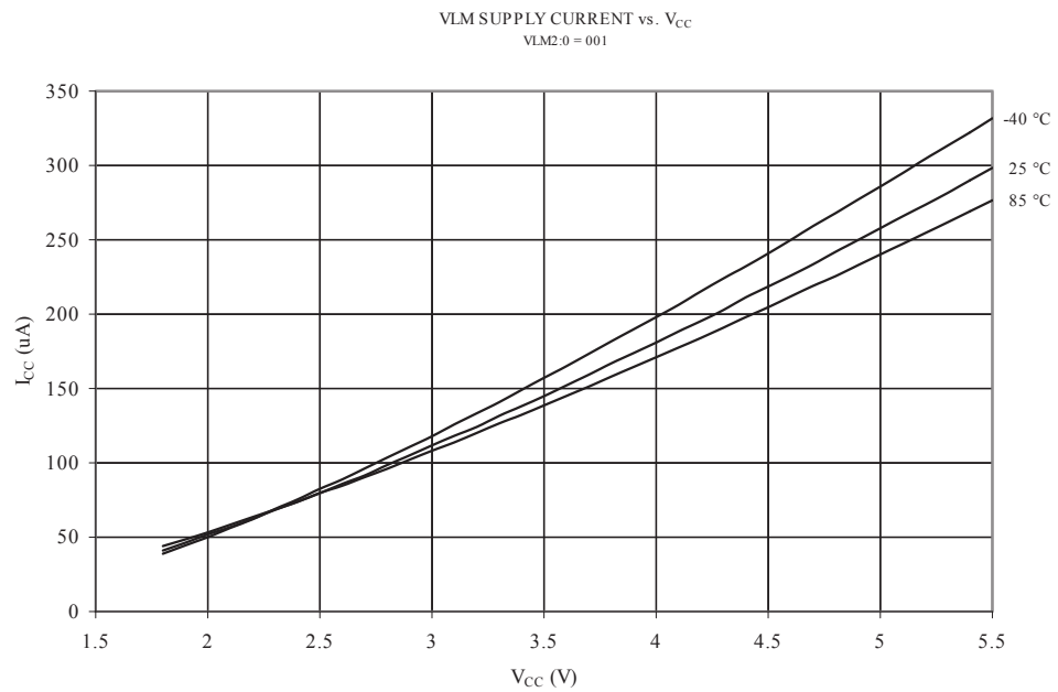
Figure 19-49 Temperature Dependence of VLM Current vs. V_{CC}
