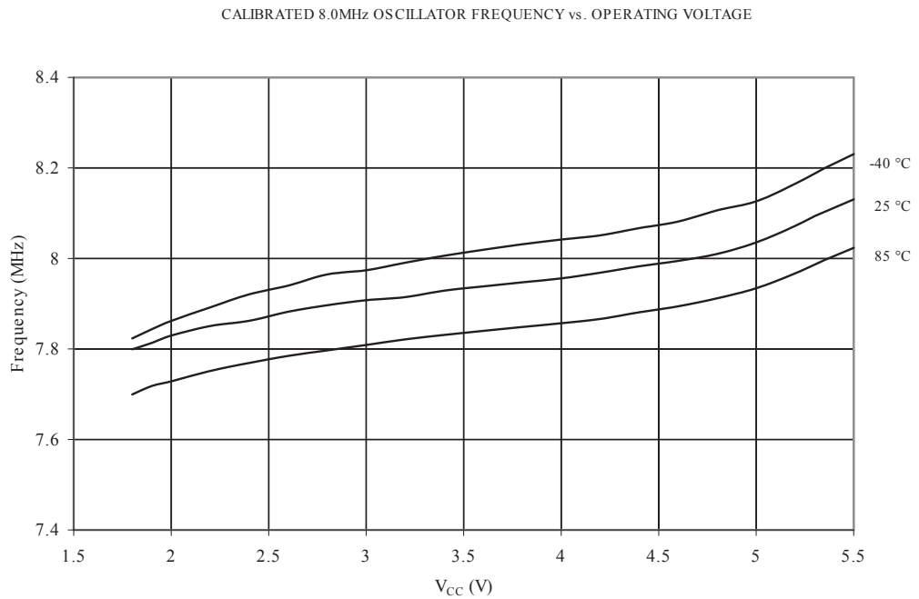
Figure 19-39 Calibrated Oscillator Frequency vs. V_{CC}
