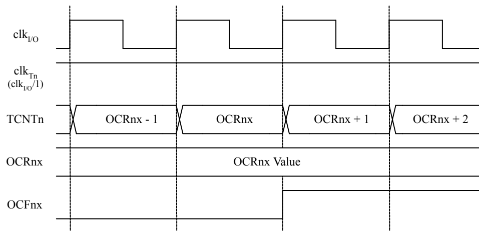
Figure 13-12 Timer/Counter Timing Diagram, Setting of OCF0x, no Prescaling
