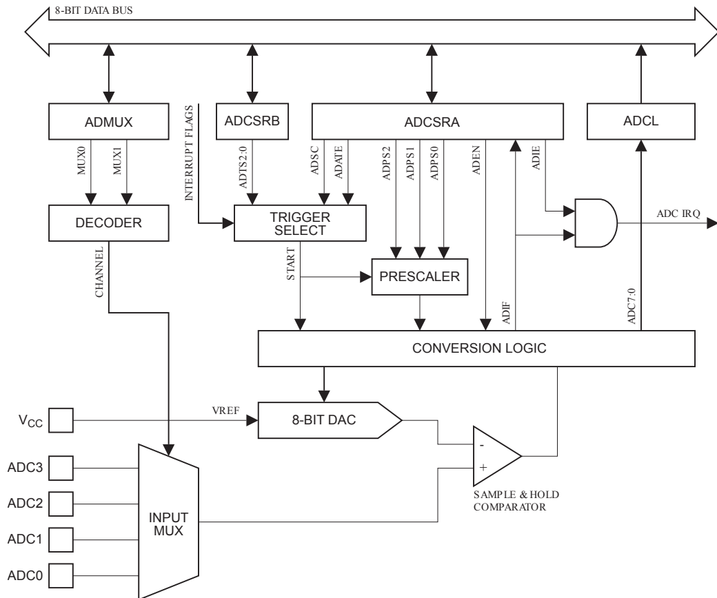
Figure 15-1 Analog to Digital Converter Block Schematic Operation
