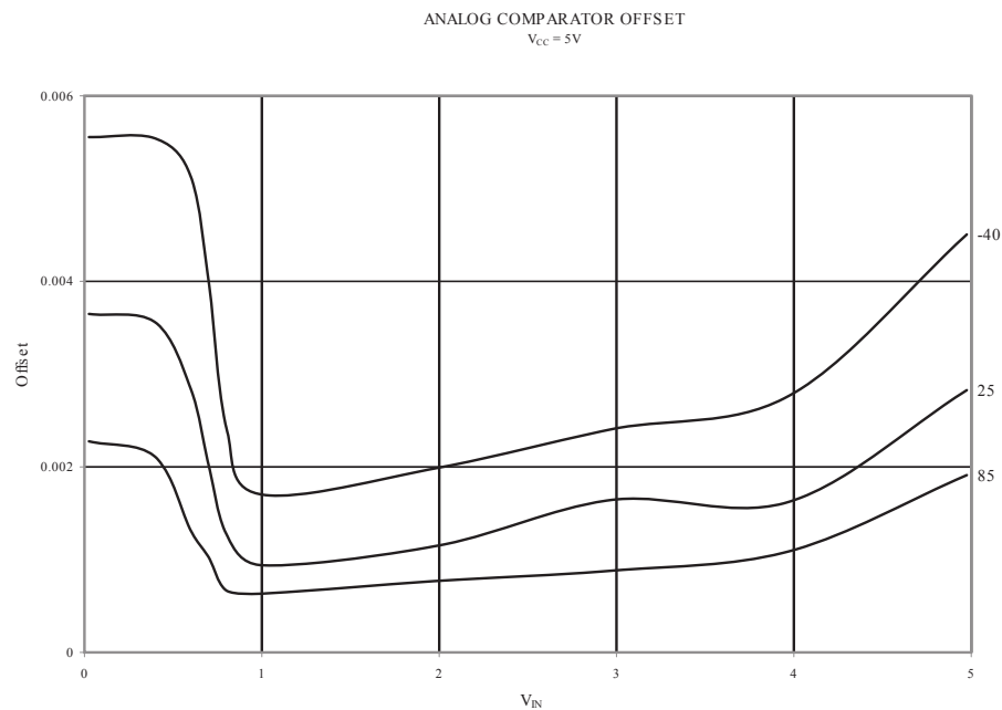
Figure 19-36 Analog Comparator Offset
