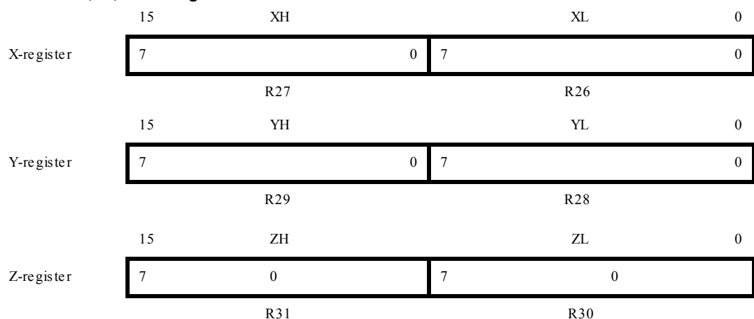
Figure 5-3 The X-, Y-, and Z-registers
