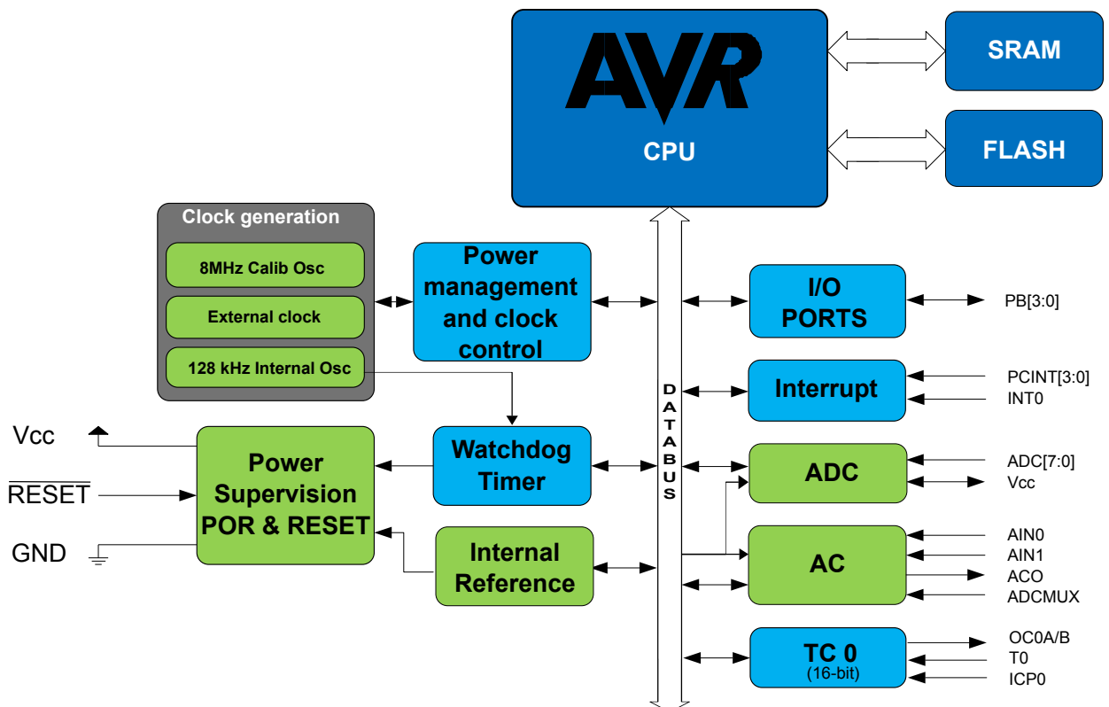
Figure 3-1 Block Diagram
