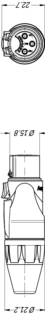
FEMALE CONNECTOR 1:1
