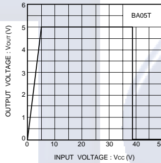
Fig. 10 Over voltage protection characteristics
