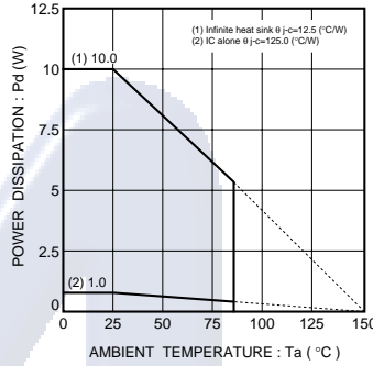
Fig. 7 Ta - power dissipation characteristics (TO 252-3)
