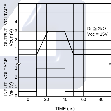
Fig.9 Output response characteristics
