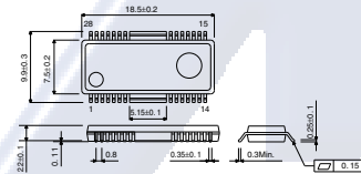
HSOP-M28
