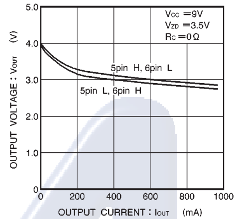
Fig.15 Output voltage vs. output current
