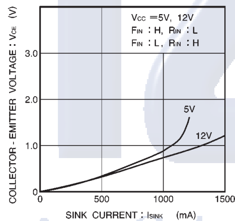
Fig.8 Output saturated voltage vs. sink current ( I )
