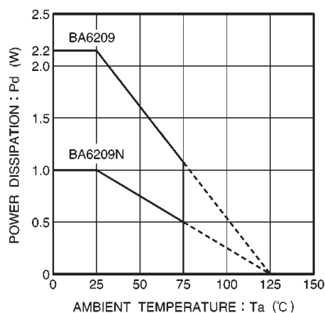
Fig.1 Temperature dependence power dissipation curves
