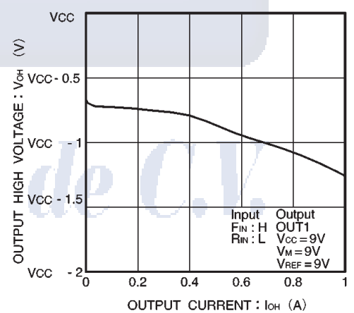
Fig.8 Output high level voltage vs. output current
