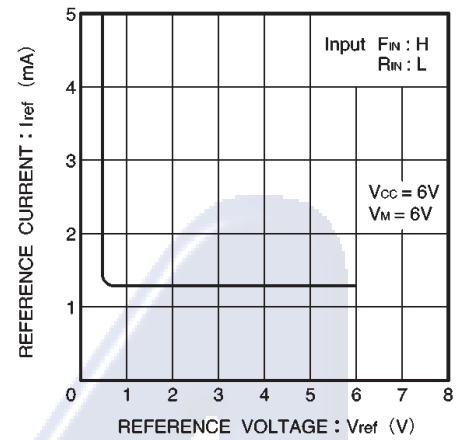
Fig.11 V_{ref} reference current vs. V_{ref} reference voltage
