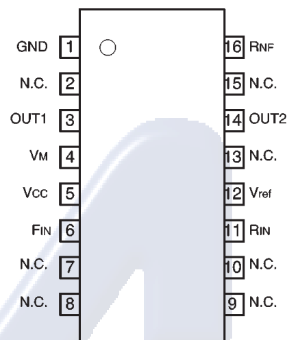
Fig.1 Pin assignments
