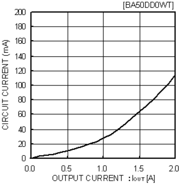
Fig.22 Circuit Current by Load Level ( I_{OUT}=0\text{mA}\rightarrow 2\text{A} )
