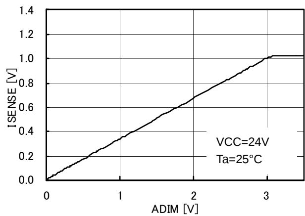
Figure 11. ISENSE feedback voltage v.s. ADIM
