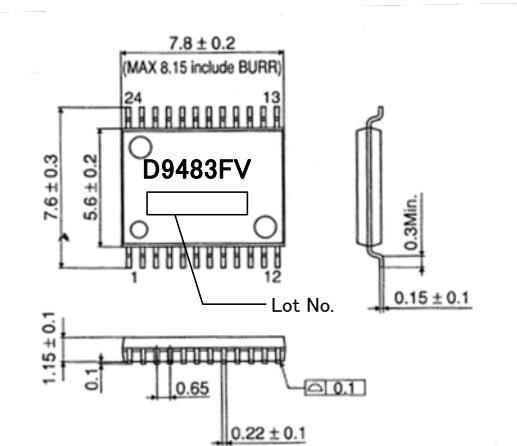
Figure 4-2. SSOP-B24
