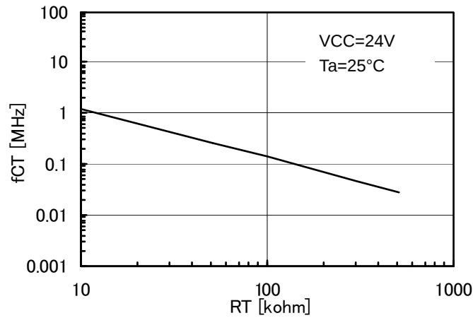
Figure 8. f_{CT} v.s. R_T
