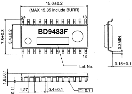
Figure 4-1. SOP-24
