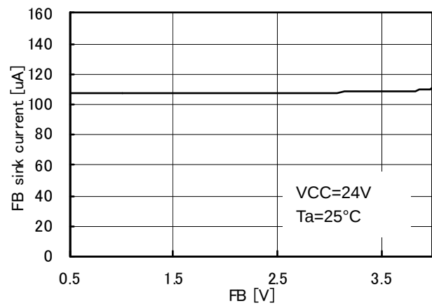
Figure 9. FB sink current v.s. FB voltage
