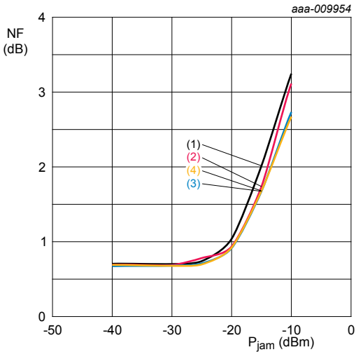
f_{jam} = 850 \text{ MHz} ; T_{amb} = 25 \text{ }^{\circ}\text{C} ; f = 1575 \text{ MHz} ; including PCB losses. 1. V_{CC} = 1.5 \text{ V} 2. V_{CC} = 1.8 \text{ V} 3. V_{CC} = 2.85 \text{ V} 4. V_{CC} = 3.1 \text{ V}
