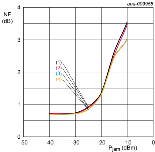
f_{jam} = 1850 \text{ MHz} ; T_{amb} = 25 \text{ }^{\circ}\text{C} ; f = 1575 \text{ MHz} ; including PCB losses. 1. V_{CC} = 1.5 \text{ V} 2. V_{CC} = 1.8 \text{ V} 3. V_{CC} = 2.85 \text{ V} 4. V_{CC} = 3.1 \text{ V}
