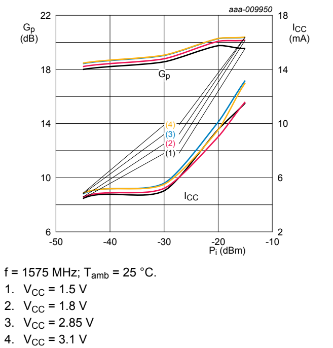
Figure 8. Power gain and supply current as function of input power; typical values
