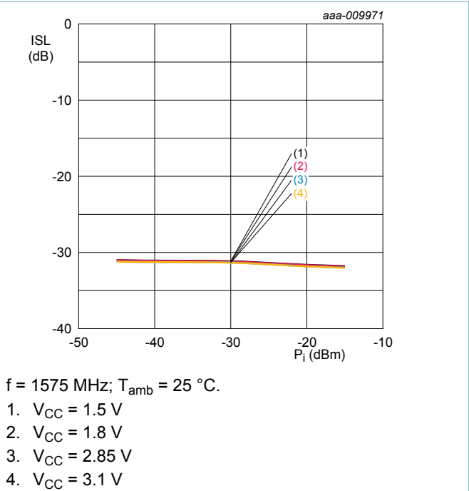
Figure 25. Isolation as a function of input power; typical values
