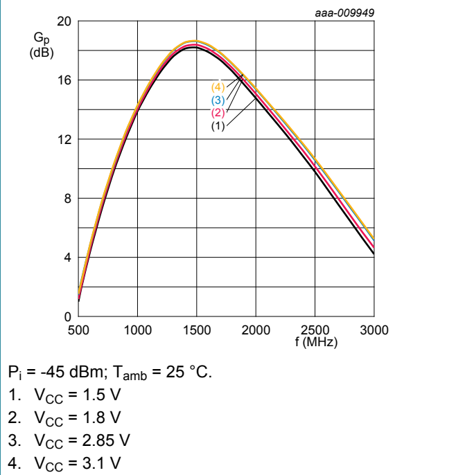
Figure 7. Power gain as a function of frequency; typical values
