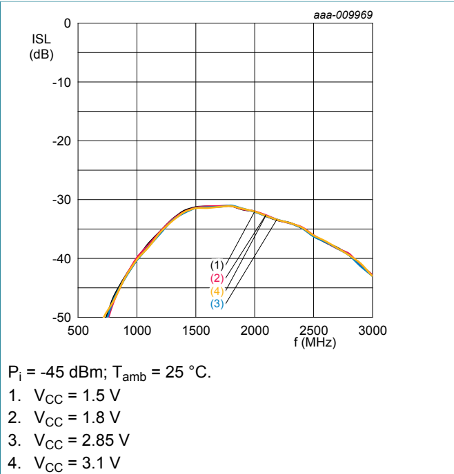
Figure 24. Isolation as a function of frequency; typical values
