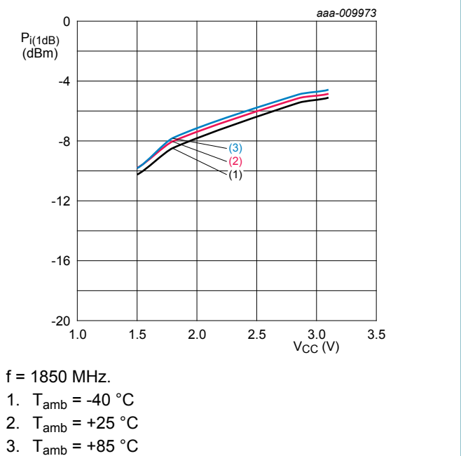
Figure 27. Input power at 1 dB gain compression as a function of supply voltage; typical values
