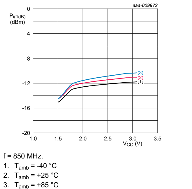
Figure 26. Input power at 1 dB gain compression as a function of supply voltage; typical values
