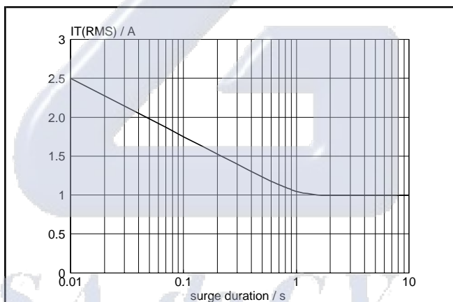
Fig. 5. Maximum permissible repetitive rms on-state current I_{T(RMS)} , versus surge duration, for sinusoidal currents, f = 50\text{ Hz} ; T_{lead} \leq 51^\circ\text{C} .
