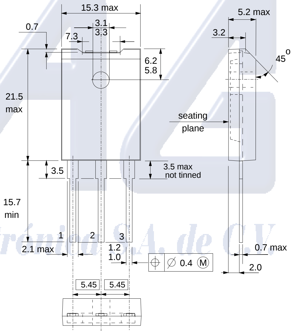
Fig.15. SOT199; The seating plane is electrically isolated from all terminals.
