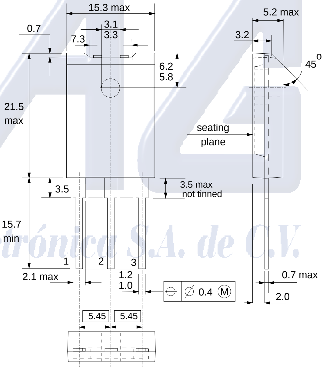
Fig.12. SOT199; The seating plane is electrically isolated from all terminals.
