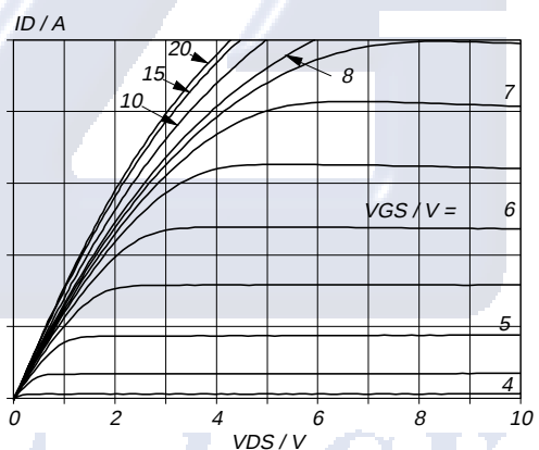
Fig.5. Typical output characteristics, T_j = 25\text{ }^\circ\text{C} . I_D = f(V_{DS}) ; parameter V_{GS}
