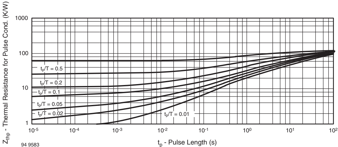
Fig. 5 - Thermal Response
