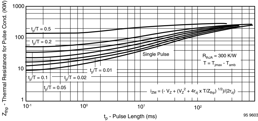
Fig. 13 - Thermal Response
