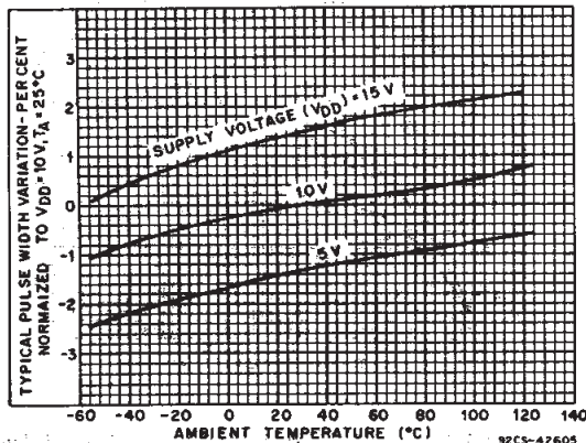
Fig. 10 - Typical pulse-width variation as a function of temperature (R X = 100 KΩ, C X = 0.1 μF).
