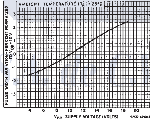
Fig. 9 - Typical pulse-width variation as a function of supply voltage.
