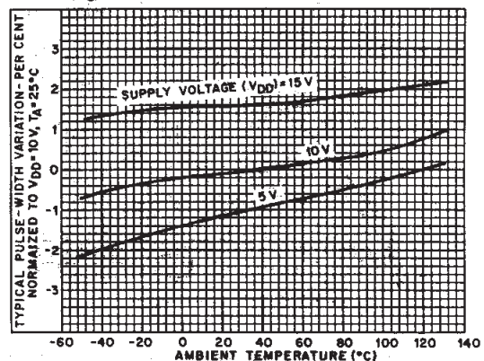
Fig. 11 - Typical pulse-width variation as a function of temperature (R X = 100 KΩ, C X = 2000 pF).
