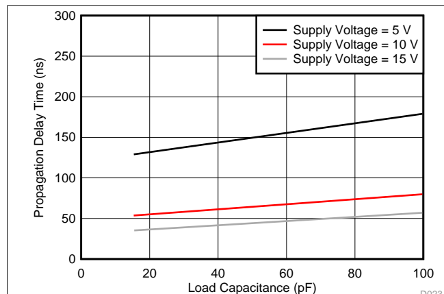
Figure 5. Typical Propagation Delay Time vs Load Capacitance
