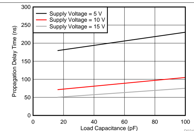
Figure 6. Typical Propagation Delay Time vs Load Capacitance
