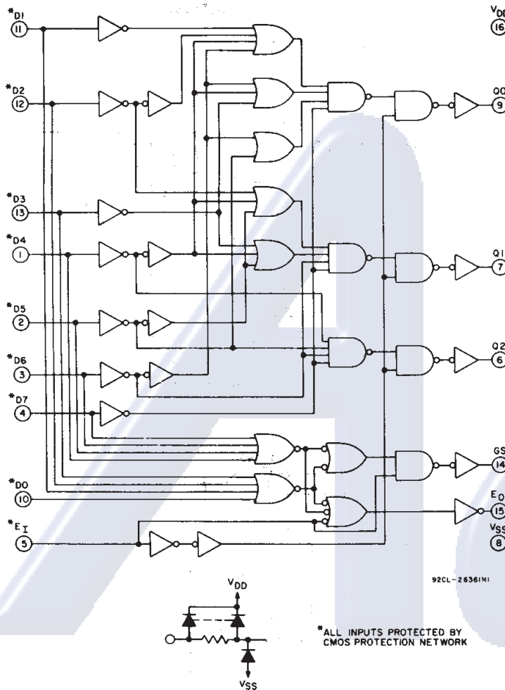
Fig. 8 - CD4532 logic diagram.
