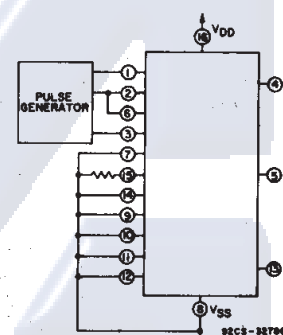
Fig. 23—Functional test circuit.
