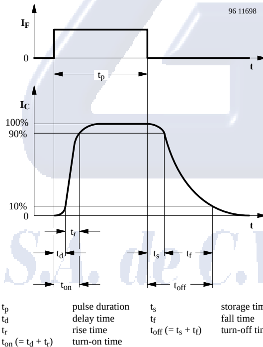
Figure 3. Switching times
