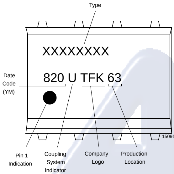
Figure 14. Marking example
